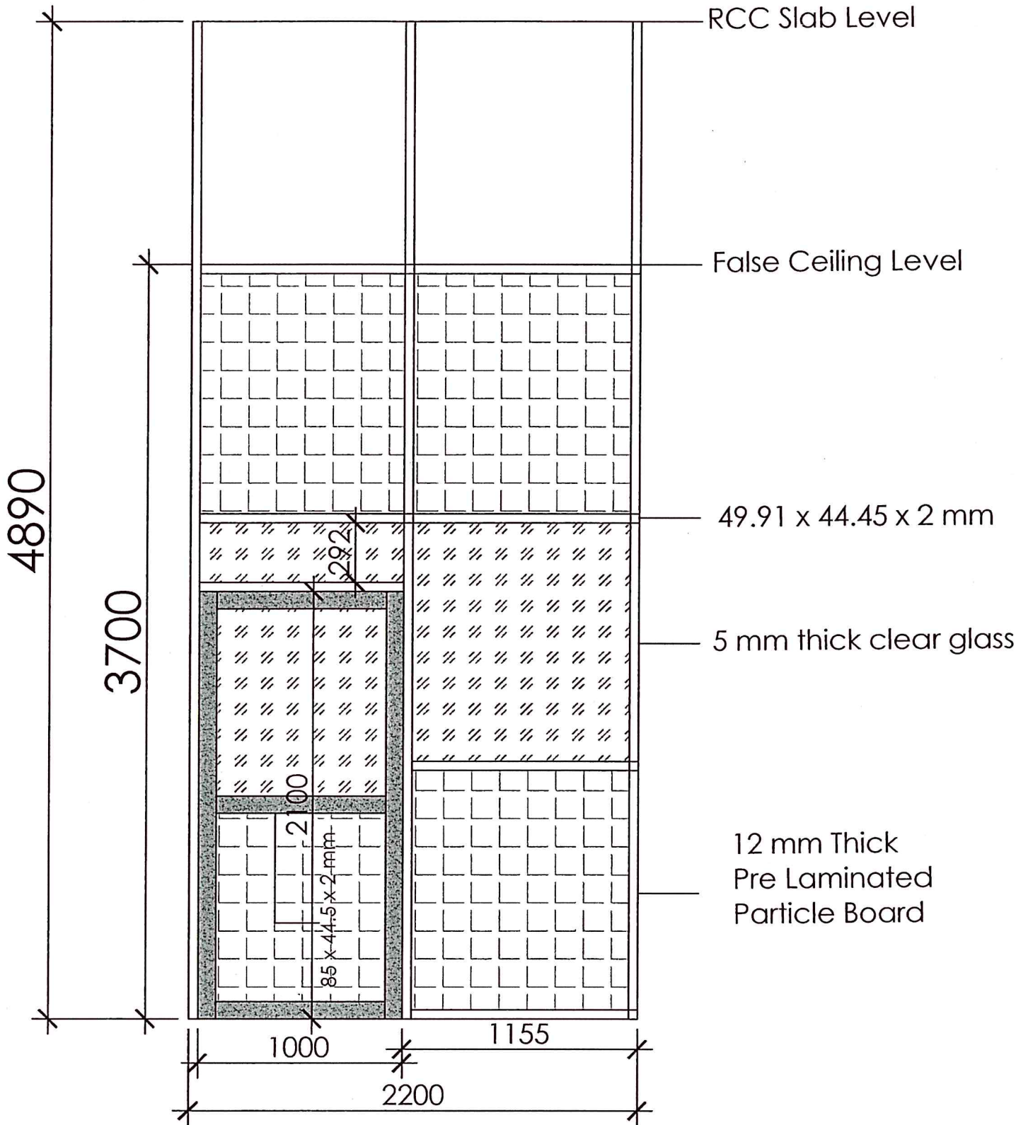
Elevation (B) of Aluminium Partition Work
